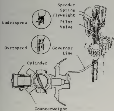
FIGURE 7-13. On-speed, basic operation.
